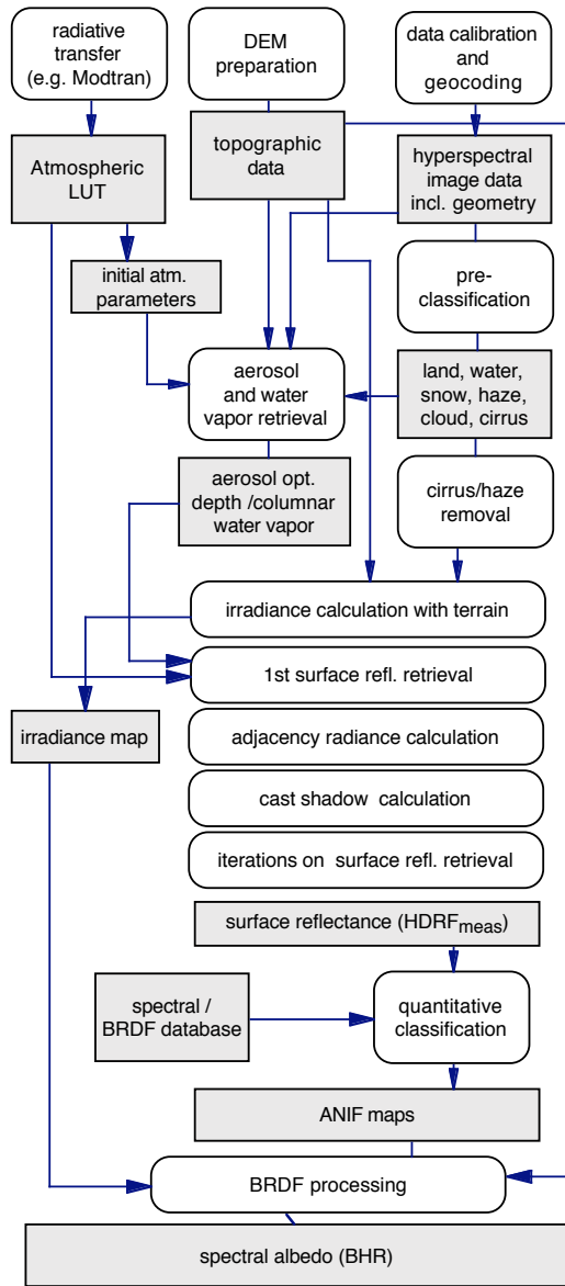
Figure 1: Complete atmospheric correction and radiometric normalization scheme.
