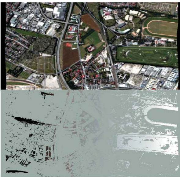
Figure 10 Results of BRDF correction using measured BRDF values (top: corrected image, bottom: anisotropy factor for the lawn object).
