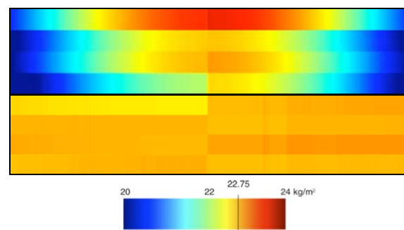
Figure 8 Water vapor retrieval over 8 different targets without smile correction (top), and with smile correction (bottom).
